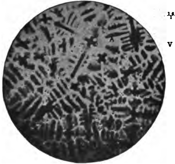
Fig. 36. Alloy of 97.1 per cent Copper, 2.9 per cent Aluminium showing Heterogeneous of Solid Solution.
